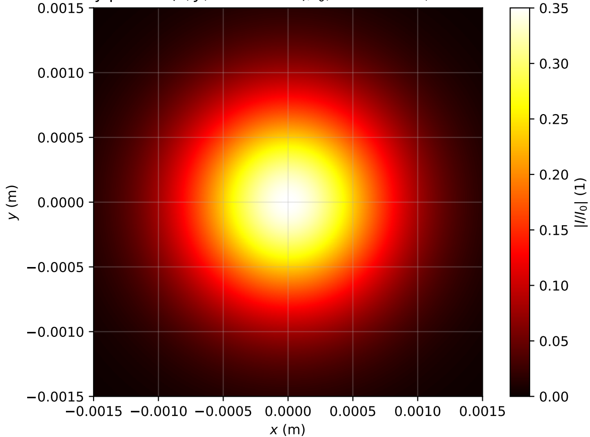
Intensity profile I(x, y, z = 3.821m)/I_0 , P_{in}=0.4P_{cr} , artificial time
